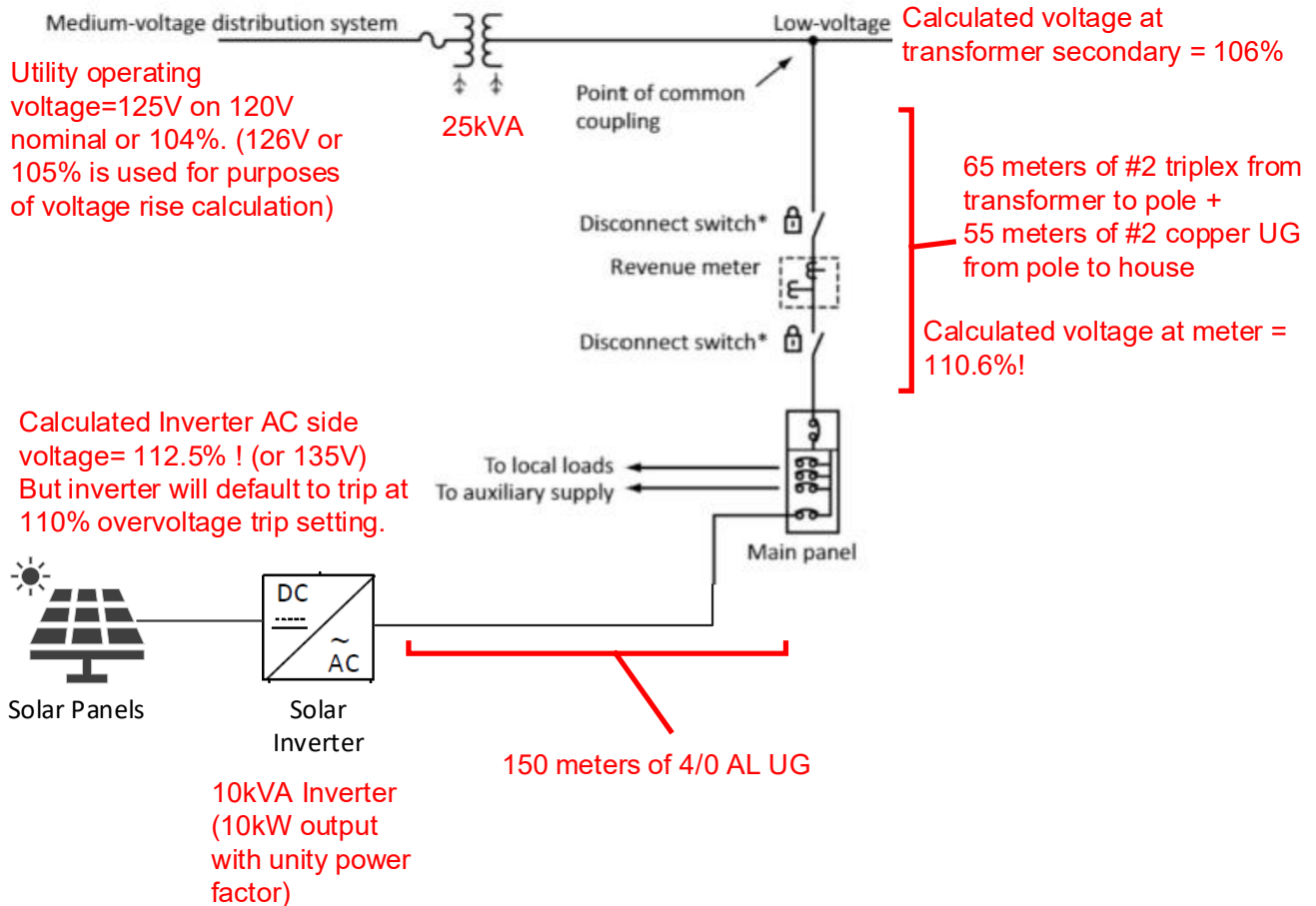
Figure 3 - Secondary voltage rise example with small MG system
