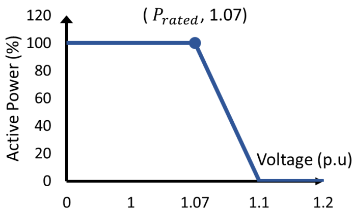
Figure 2 – Default Volt Watt Control Curve.
